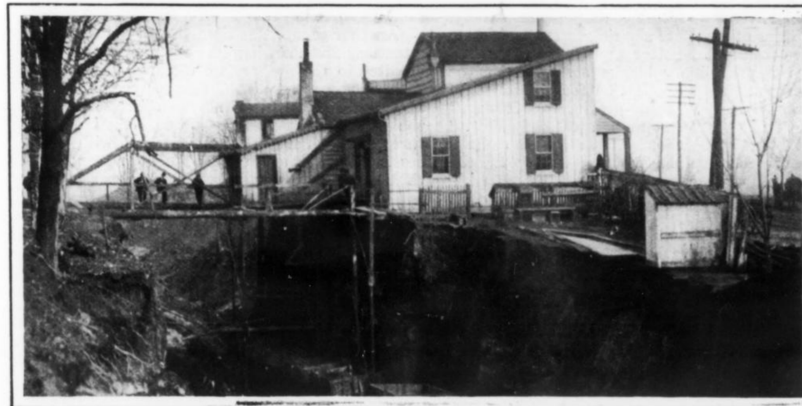
(PRIZE WINNER, $10.) A HOUSE IN MID-AIR—DWELLING AT WESTPORT, MD., UNDERMINED BY A CUT FOR A NEW RAILROAD, AND PROPPED UP TO PREVENT COLLAPSE. Mrs. C. R. Miller, Maryland.
