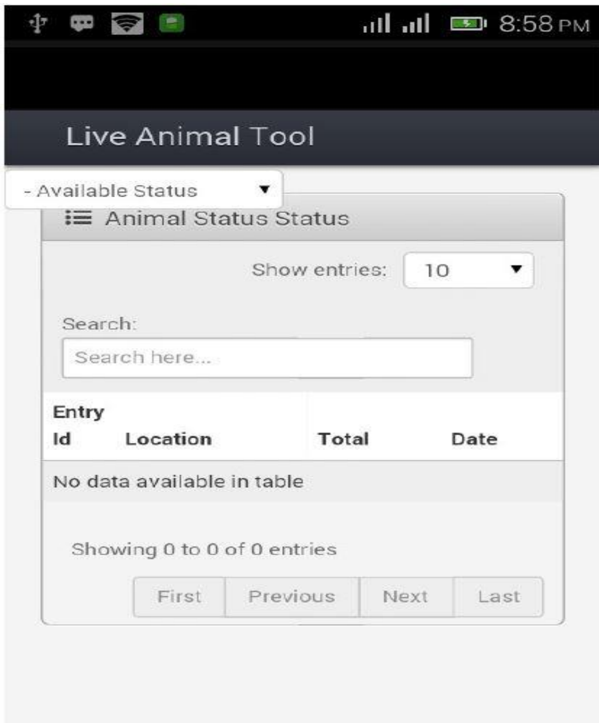
Figure 31: Report Generation
