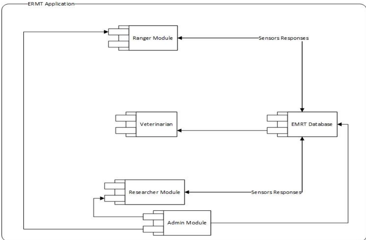
Figure 23: Component diagram
