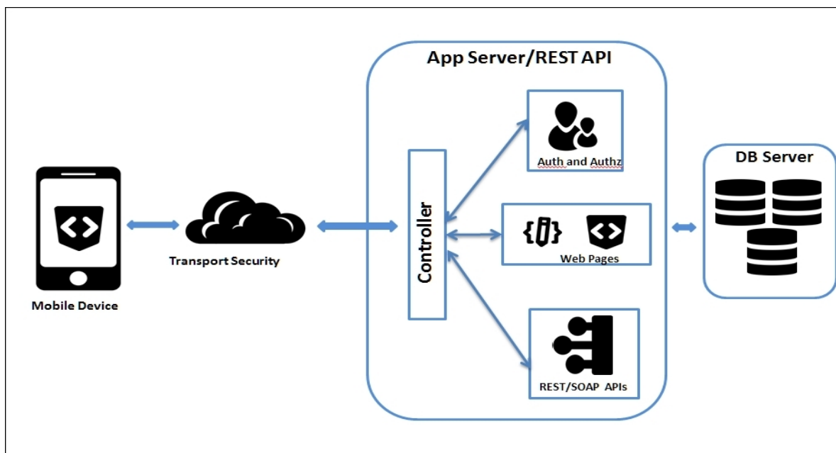
Figure 22: Architecture Diagram
