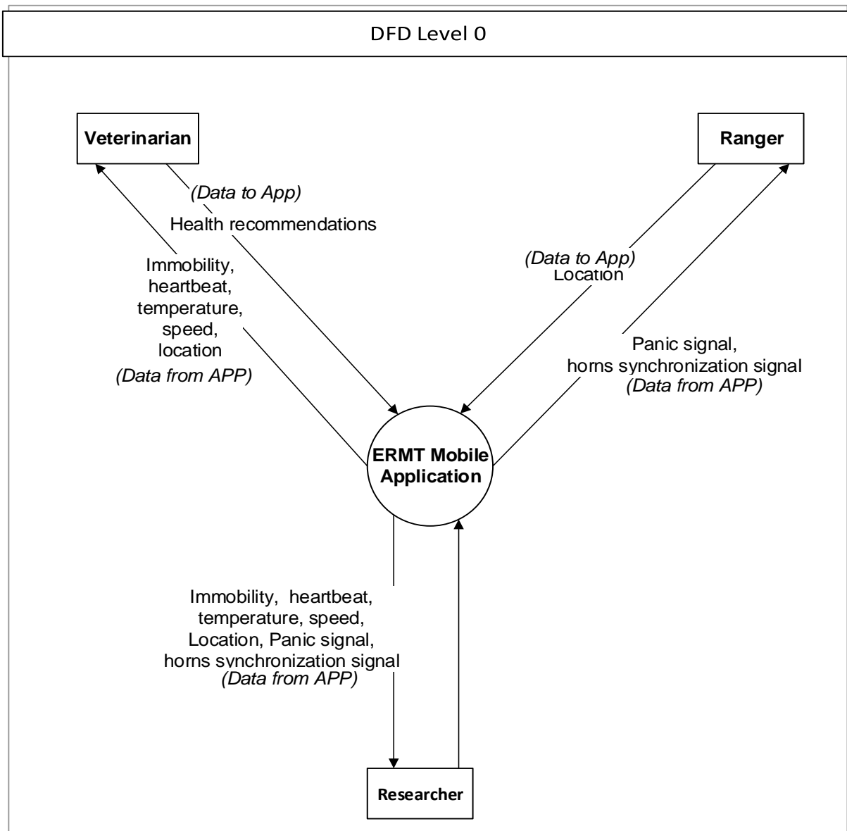
Figure 24: Data Flow Diagram
