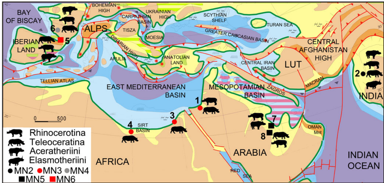
Figure 6. Early Miocene paleogeographic map (modified from Popov et al., 2004) showing selected localities mentioned in the text. (1) The Negev, early Miocene, MN3, Israel; (2) Bugti Hills (Upper Member of Chitarwata Formation), early Miocene, MN2, Pakistan; (3) Moghara, early Miocene, MN3, Egypt; (4) Jebel Zelten, early Miocene, MN3, Libya; (5) Sansan, middle Miocene, MN6, France; (6) Bézian-La Romieu, late early Miocene, MN4, France; (7) Al-Sarrar, middle Miocene, MN5, Saudi Arabia; (8) Ad Dabtiyah, middle Miocene, MN5, Saudi Arabia. The Rhinocerotidae taxa for each locality are listed in Table 1. Mnt = Mountain.
