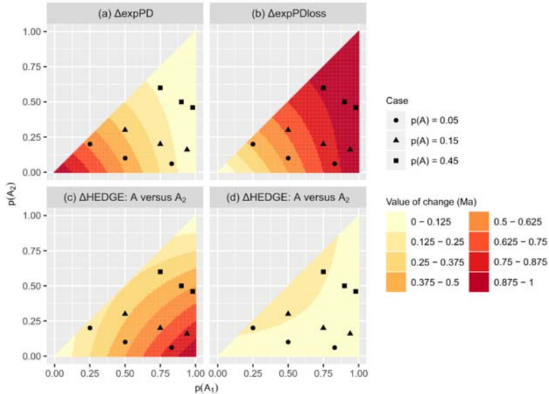
Fig. 2. Values of change due to the split of species A into two sister species A_1 and A_2 with respect to the extinction probability of A_1 ( p(A_1) ), and the extinction probability of A_2 ( p(A_2) ) in (a) the expected phylogenetic diversity ( expPD ), (b) the expected loss of phylogenetic diversity ( expPDloss ) of the tree, (c) in the HEDGE score of species A by comparing HEDGE score of A at t to HEDGE score of A_1 (the more threatened post-split species) at t' and (d) in the HEDGE score of species A by comparing HEDGE score of A at t to HEDGE score of A_2 (the less threatened post-split species) at t' . These values are represented for an arbitrary age of post-split species \theta = 1 Ma. Dots represent numerical applications for the six case studies described in Table 1. Note that the values of change in expPDloss ( \Delta expPDloss ) are equal to the values of change in the HEDGE score of species A when comparing HEDGE score of A at t to HEDGE score of ( A_1, A_2 ) at t' .
