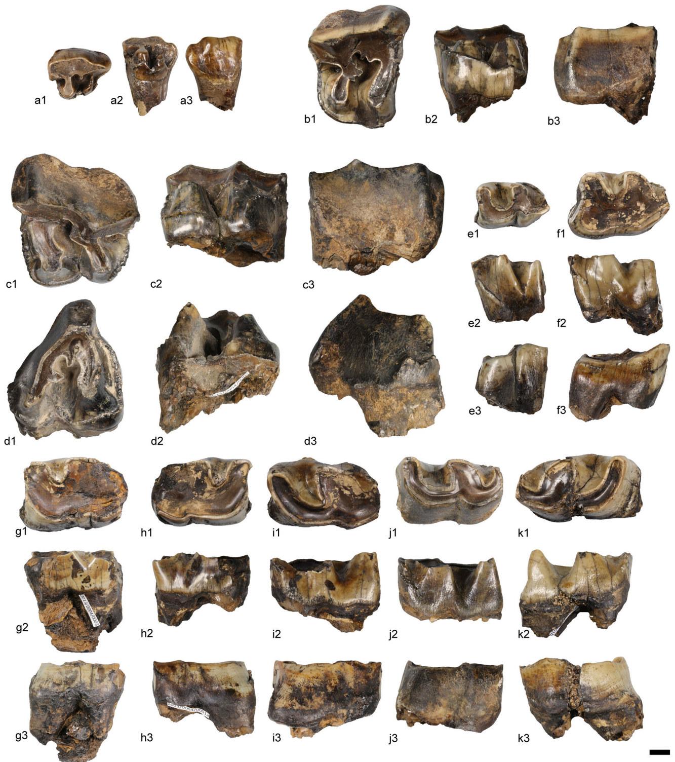
Fig. 1 Brachypotherium brachypus from Gračanica (early middle Miocene, Bugojno Basin, Bosnia-Herzegovina). a Right P1 (NHMW 20013/0003/0011) in occlusal (a1), lingual (a2) and labial (a3) views. b Right P4 (NHMW 2013/0004/0007) in occlusal (b1), lingual (b2) and labial (b3) views. c Left M2 (NHMW 2013/0004/0006) in occlusal (c1), lingual (c2) and labial (c3) views. d Right M3 (NHMW 2013/0004/0005) in occlusal (d1), lingual (d2) and labial (d3) views. e Right p3 (NHMW 2013/0003/0004) in occlusal (e1), lingual (e2) and labial (e3) views. f
