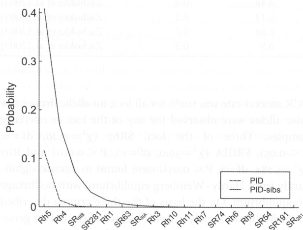
FIG. 2 Cumulative values of probability of identity and probability of identity among siblings for 17 microsatellite loci screened on 10 reference samples of rhinoceros dung.
