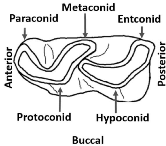
Figure 1: Schematic of the five major cusps on a m2 of a rhinoceros. Protoconids and hypoconids display both Phase 1 and Phase 2 facets, while paraconids, metaconids, and entoconids only display Phase 2 facets.
