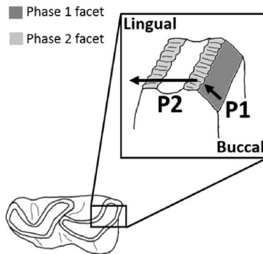
Figure 2: Schematic showing the motion and both phases of the chewing stroke in rhinoceroses. Phase 1 facets occur as flattened, inclined planes, while Phase 2 facets occur as horizontal planes with the wavy texture of HSB.
