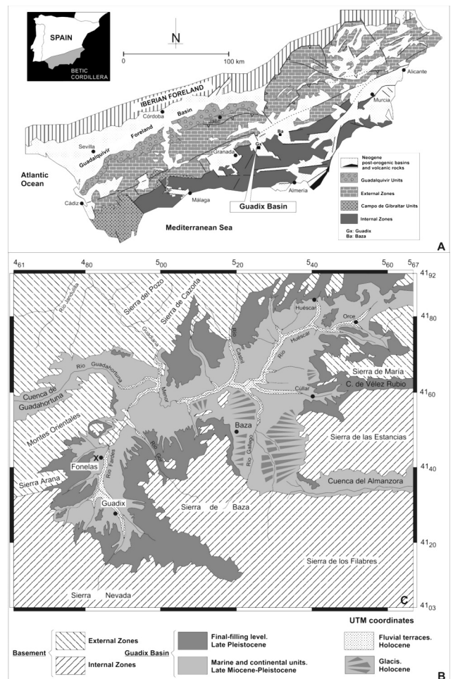
Fig. 1. Geological maps of the Betic Cordillera and Guadix Basin. The location of Fonelas P-1 large mammals site, close to the Fonelas village, is indicated in the lower map (from Viseras et alii , 2006).
