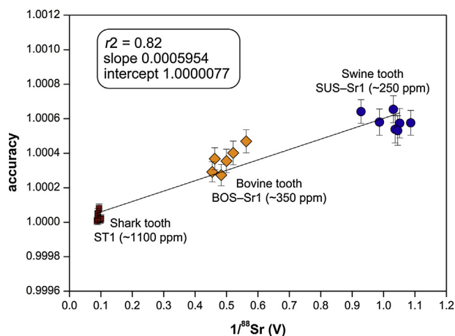
Fig. 4. Correlation between the accuracy of the ^{87}\text{Sr}/^{86}\text{Sr} analysis (observed/true) and the inverse of the ^{88}\text{Sr} signal. This high correlation is attributed by some authors to the Ca–P–O interference which occurs during LA analysis of bioapatites (see text for details). The line equation is used to correct our LA data.
