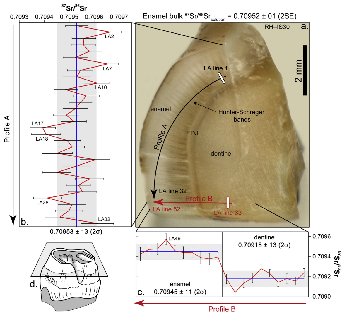
Fig. 1. a. RH-IS30 sample photo, with visible Hunter-Schreger bands. b. Profile A is composed by 32 small ( 100 \times 500 \mu\text{m} ) LA analyses; blue line is the average of the analyses; grey area is the 2\sigma -error of 0.00008 calculated from the standard materials; x-error bars are the 2-standard errors. c. Profile B starts from the dentine and proceeds outward to the OES; while for enamel the profile follows the tooth growth, for dentine the direction is inverted (see text for details); symbols are the same as in profile A. d. Example of a tooth horizontal section (redrawn from [2]). (For interpretation of the references to color in this figure legend, the reader is referred to the web version of this article.)
