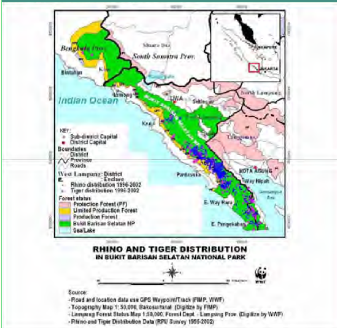
Map 3. Distribution of Rhino, and Tiger in the BBSNP
