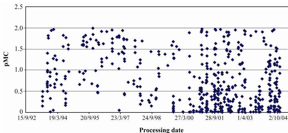
Figure 1 ORAU bone pMC values <2.0 plotted against processing date. There is a change in the distribution at 8/2000 (see text for details). One additional reason for the increasing number of determinations <0.4 pMC is that many of the dated bones are from northern temperate and sub-arctic locations, such as Alaska and Siberia, where preservation of bone collagen is favored generally by lower temperatures and permafrost conditions, and extractable yields are therefore higher.
