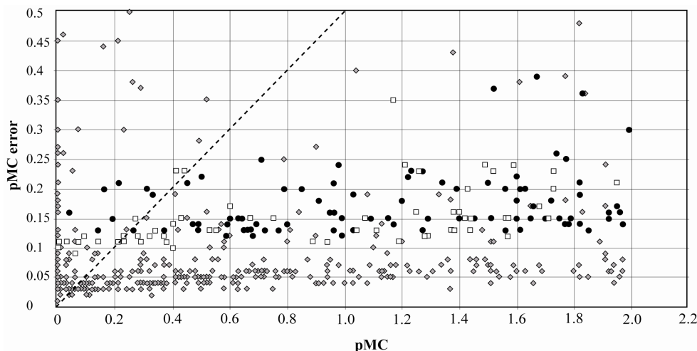
Figure 2 pMC plotted against pMC error. Each point is a ^{14}\text{C} measurement in pMC dated at ORAU over the last 15 yr <2 pMC. The dashed line represents “pMC error \times 2 ,” which defines T_{\text{max}} . pMC values to the left of this line are “greater than” ages. To obtain finite AMS age determinations >50 kyr BP, a precision of \pm 0.1 pMC is required. The diamonds are ultrafiltered gelatin determinations. This figure shows an increase in the number of these compared with other measurements of ion exchanged (black circles) and gelatin determinations (open squares). Our conclusion is that this is due principally to 1) the increased levels of measurement precision produced since the installation of the new HVEE accelerator (see text) and 2) the introduction of ultrafiltration in the routine pretreatment of bone, improving the removal of contaminants in very old bone material.
