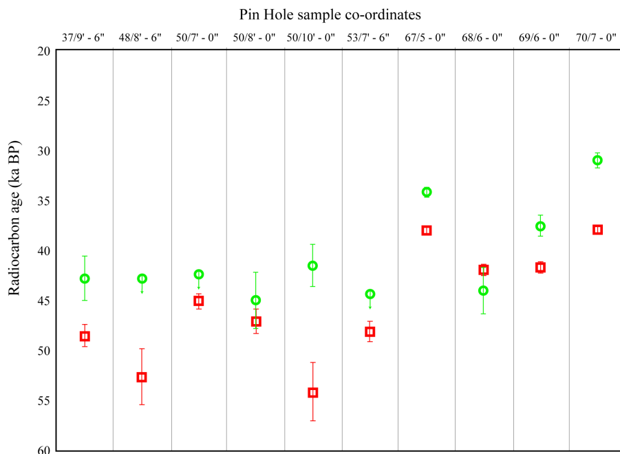
Figure 4 Comparison between initial AMS dates from Pin Hole, pretreated using ion-exchanged gelatin techniques (squares) and a new series based on ultrafiltration (circles). The results are presented in order based on distance into the cave from the datum point at the entrance.
