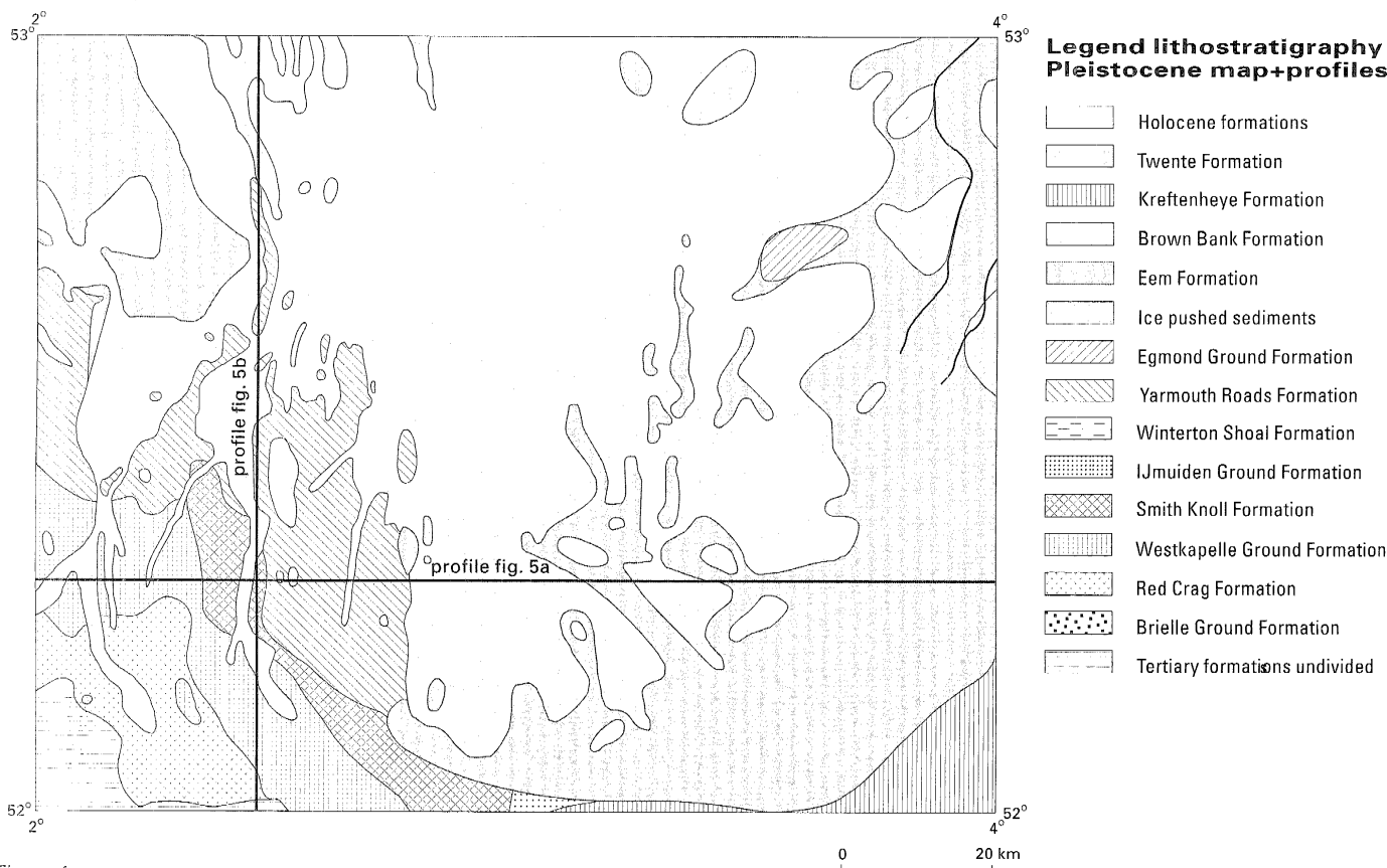
Figure 4 The lithostratigraphy of the top of the Pleistocene of the geological sheet Flemish Bight of the southern bight of the North Sea between 52° and 53°N/2° and 4° E. Location of sections shown in 5A and B.
