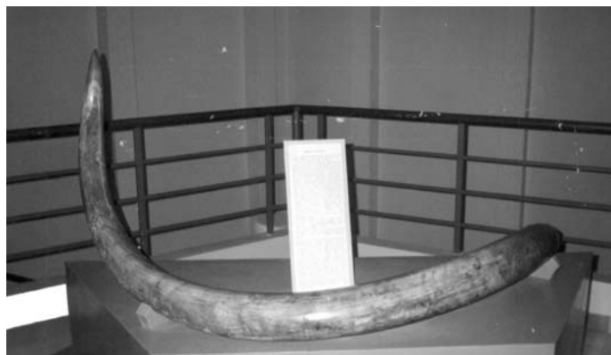
Fig 22 Large tusk of a male woolly mammoth
