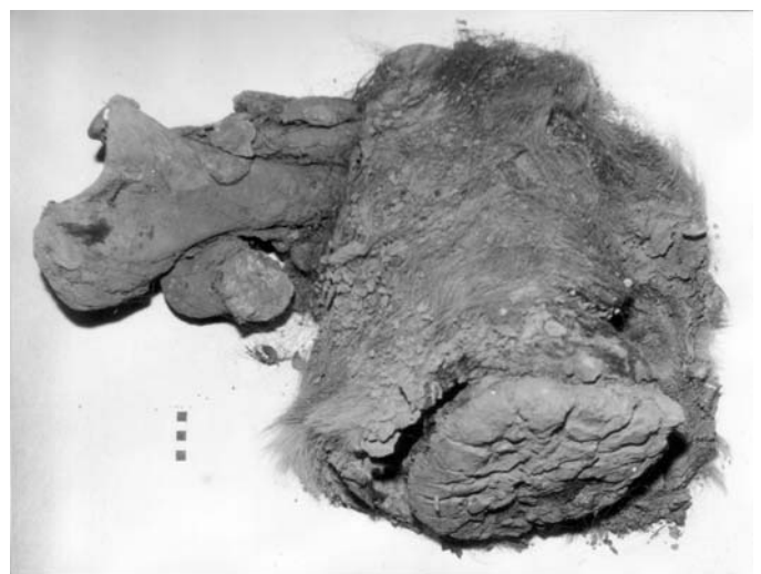
Fig 15 Part of the mammoth front leg found on the Bolshoy Lyakhovsky Island
