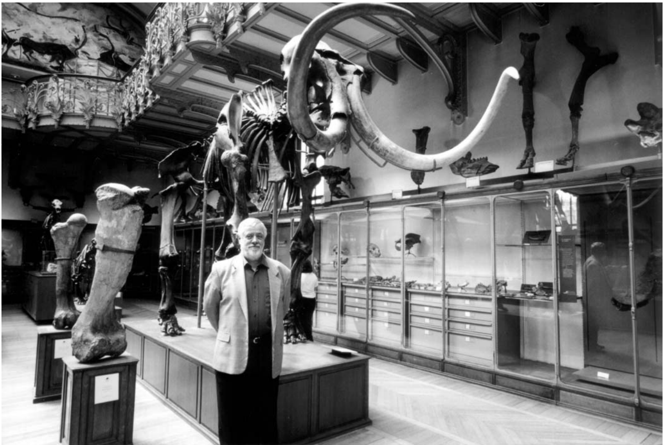
Fig 25 The complete mammoth dug out on Bolshoy Lyakhovsky Island; now in MNHN at Paris
