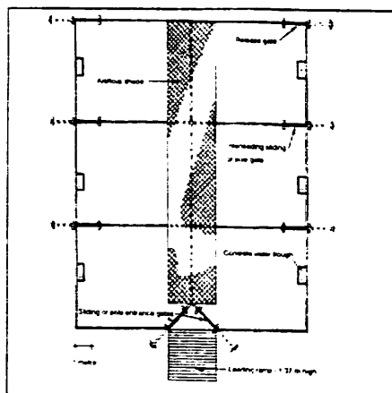
Fig. 2 - Receiving boma complex for rhinos
