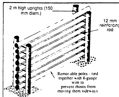
Fig. 3 - Pole gate for rhino pens
